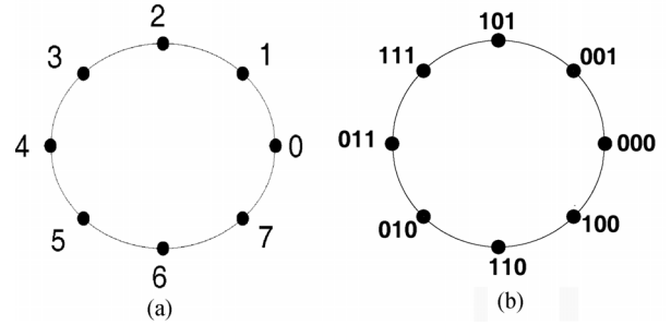
Fig. 1. The 8-PSK constellation with: (a) the isometric labeling \mu : \mathbb{Z}_8 \rightarrow \mathcal{X} ; (b) a binary labeling \eta : \mathbb{Z}_2^3 \rightarrow \mathcal{X} . The latter is a so-called Gray labeling: neighbor signals are assigned labels differing in one digit only.
