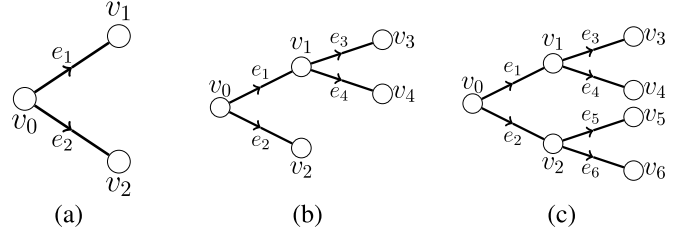
Fig. 5. d -expanded flow networks that induce flow-monotonicity of BPA routing at the root node v_0 .
