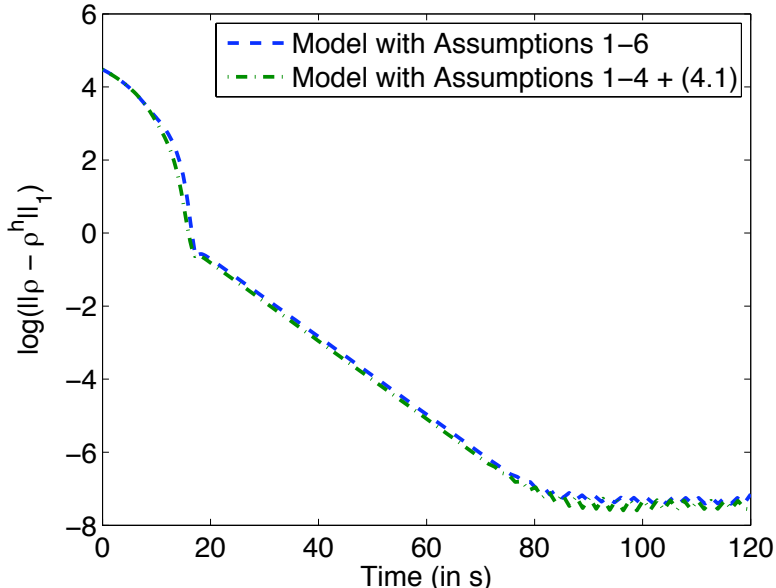
FIG. 4.2. Log-linear plot for comparison of the evolution of \|\rho(t) - \rho^h\|_1 for the local decision function of Example 3 versus the local decision function of (4.1).
