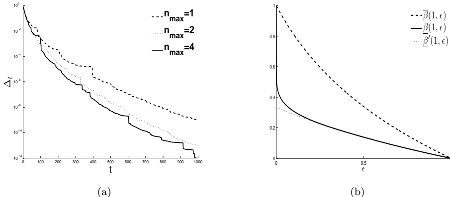
FIG. 7.1. Monte Carlo simulations of finite-window coding schemes on the BEC, with erasure probability \varepsilon = 0.5 . The performance of three coding schemes are compared: these schemes were randomly generated accordingly to (7.1) and (7.2) with n_{\max} = 1, 2, 4 respectively. In (a) the root mean squared error \Delta_t is plotted as a function of the time t in log-linear scale. In (b) -\frac{1}{\sqrt{t}} \log \Delta_t is plotted as a function of t , together with the corresponding upper bounds \sqrt{\chi_t \log \varepsilon^{-1}} provided by Theorem 5.2. The number of samples used is 200000.
