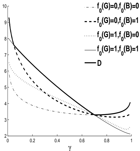
Fig. 6. The thick solid line is a plot of the Burnashev coefficient D (evaluated with natural log base) of the FSMC of Fig. 4 for the same values of the parameters as in Fig. 5.
