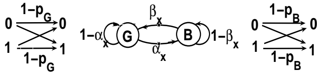
Fig. 4. a FSMC with binary state space \mathcal{S} = \{G, B\} and binary input/output space \mathcal{X} = \mathcal{Y} = \{0, 1\} : notice that the state transition probabilities are allowed to depend on the current input (ISI).
