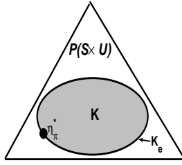
Fig. 2. A schematic representation of the optimization problem (??). The large triangular space is the infinite dimensional Prohorov space \mathcal{P}(\mathcal{S} \times \mathcal{U}) . Its gray-shaped subset represents the close convex set K of all occupation measures. The set of extreme points of K is K_e and corresponds to the set of all occupation measures associated to stationary deterministic policies. The optimal value of the linear functional \boldsymbol{\eta} \mapsto \langle \boldsymbol{\eta}, g \rangle happens to be achieved on K_e and thus corresponds to the occupation measure \boldsymbol{\eta}_{\pi^*} associated to an optimal deterministic stationary policy \pi^* : \mathcal{S} \rightarrow \mathcal{P}(\mathcal{X}) .
