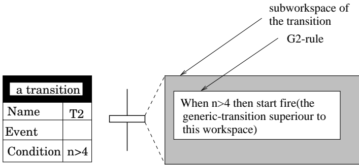
Figure 5.57 A transition, its attributes and the corresponding G2 rule.
