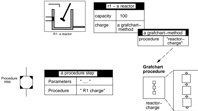
Figure 5.24 Grafchart methods.
