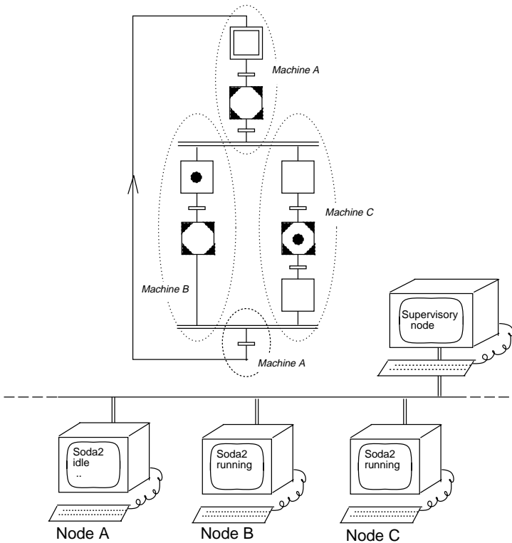
Figure 5.48 A distributed system.
