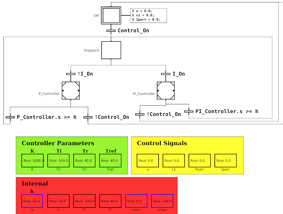
Figure 4 Contents of the PID workspace
