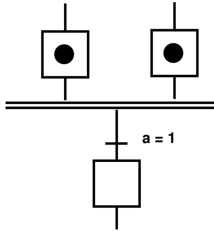
c) Firable
